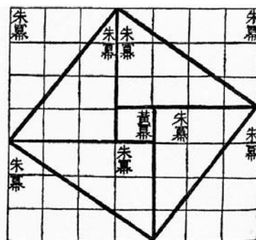
The Chinese Pythagorean theorem identified the 3-4-5 triangle in the Chou Pei Suan Ching , 500–200 B.C.E.
