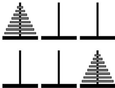
Figure 8. Towers of Hanoi: starting and target positions.
